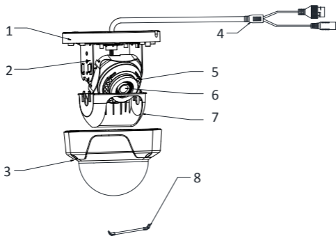
Figure 1-1 Camera Overview
