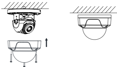
Figure 2-6 Bubble Reinstallation
